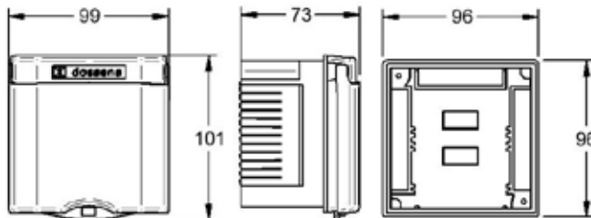
96 x 96 x 51mm - LCD display 96 x 96 x 51mm - LCD display
