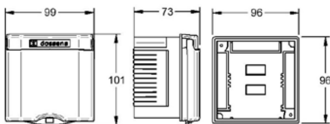
96 x 96 x 51mm - LCD display
